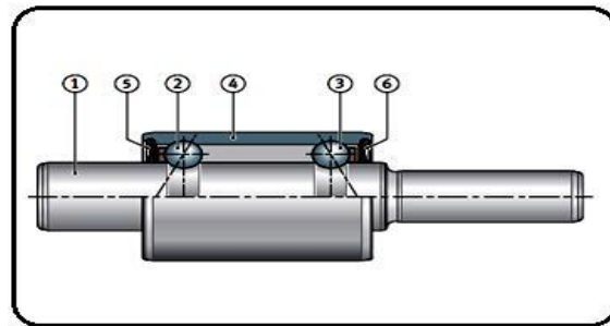
Fig 2. Mechanical water pump Bearing
